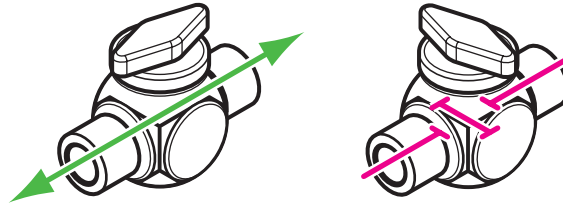
2-way with through bore
