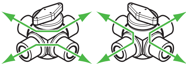
4-way with double L bore
